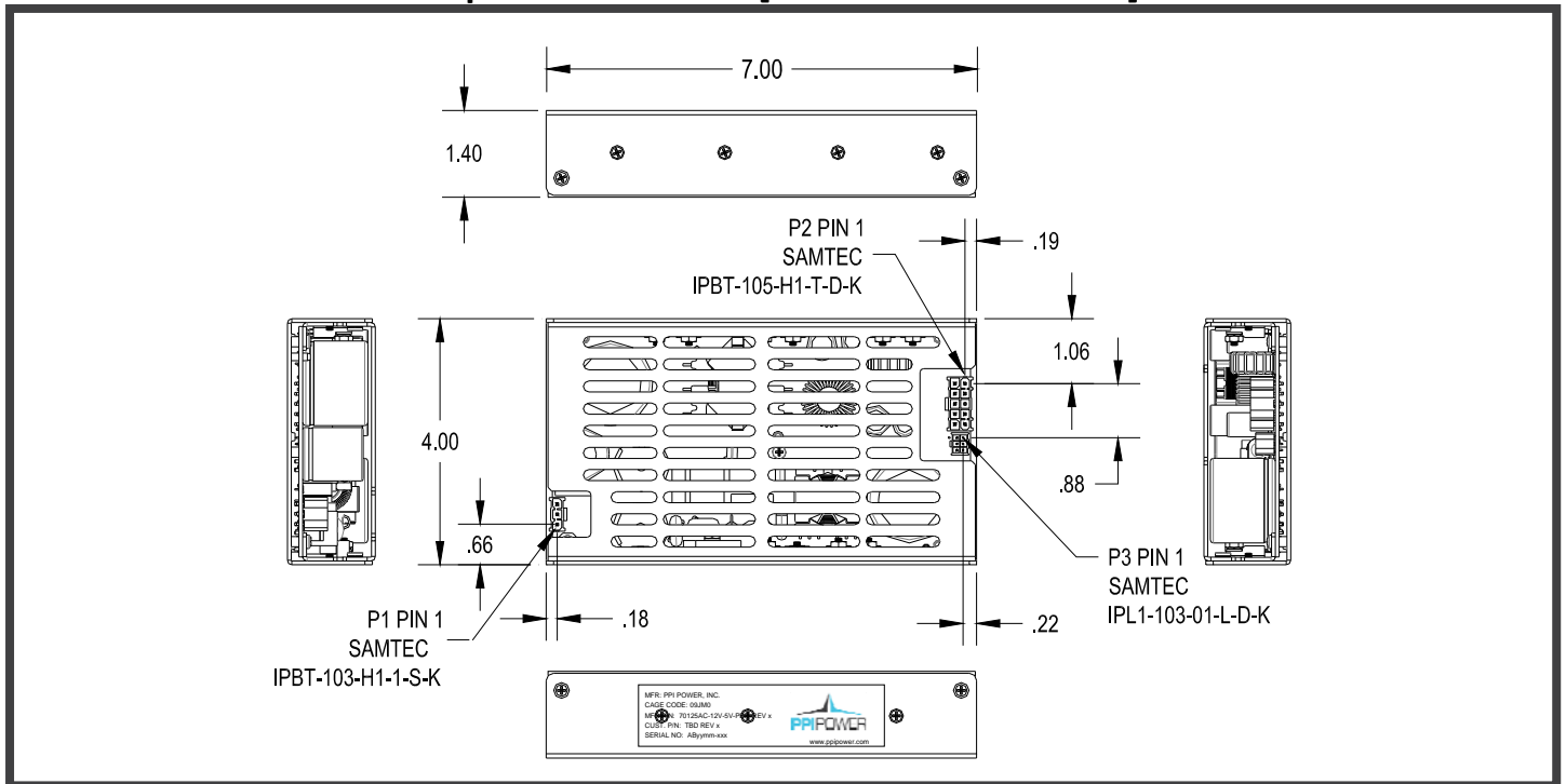
Bottom View [70125AC-12V-5V-PBF]
