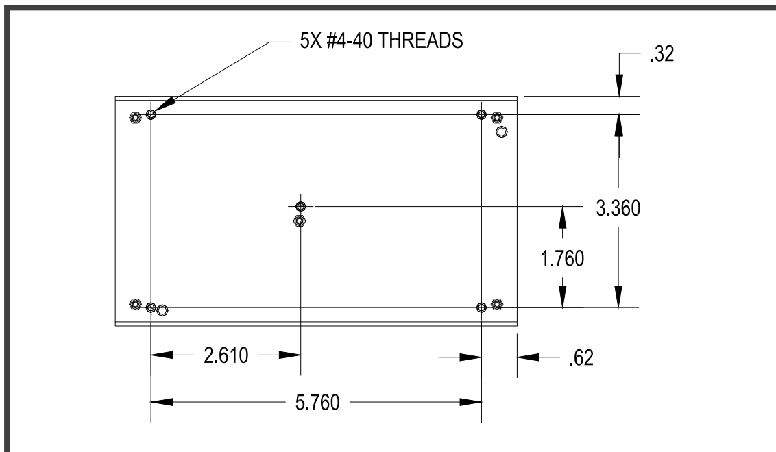
Bottom View [70125AC-12V-5V-PBF]
