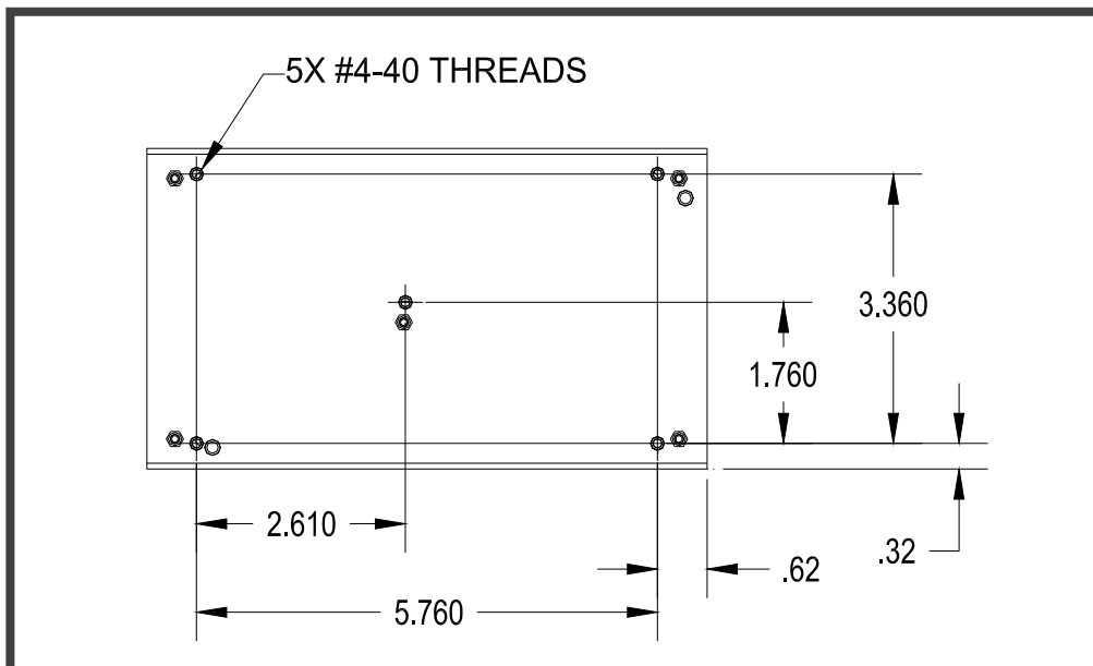
Bottom View [70125AC-12V-5V-RA-PBF]
