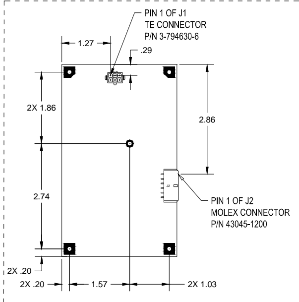
DETAIL DIMS MOUNTING HOLES AND CONNECTORS
