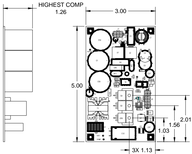
AC20W-12V-PBF (VERTICLE INTERCONNECT)
