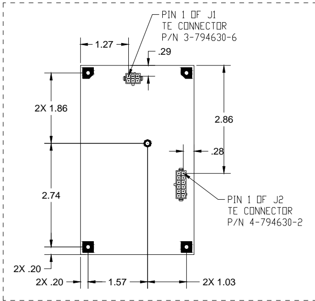
DETAIL DIMS MOUNTING HOLES AND CONNECTORS
