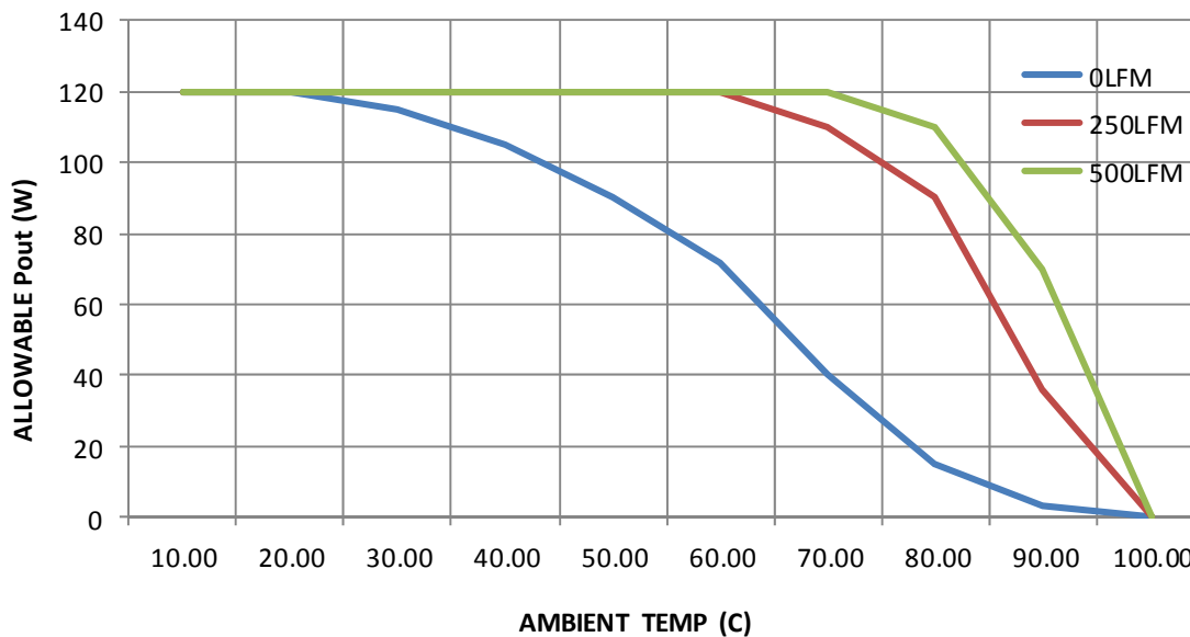
POUT VS AMBIENT TEMP - WITH HS1 HEATSINK
